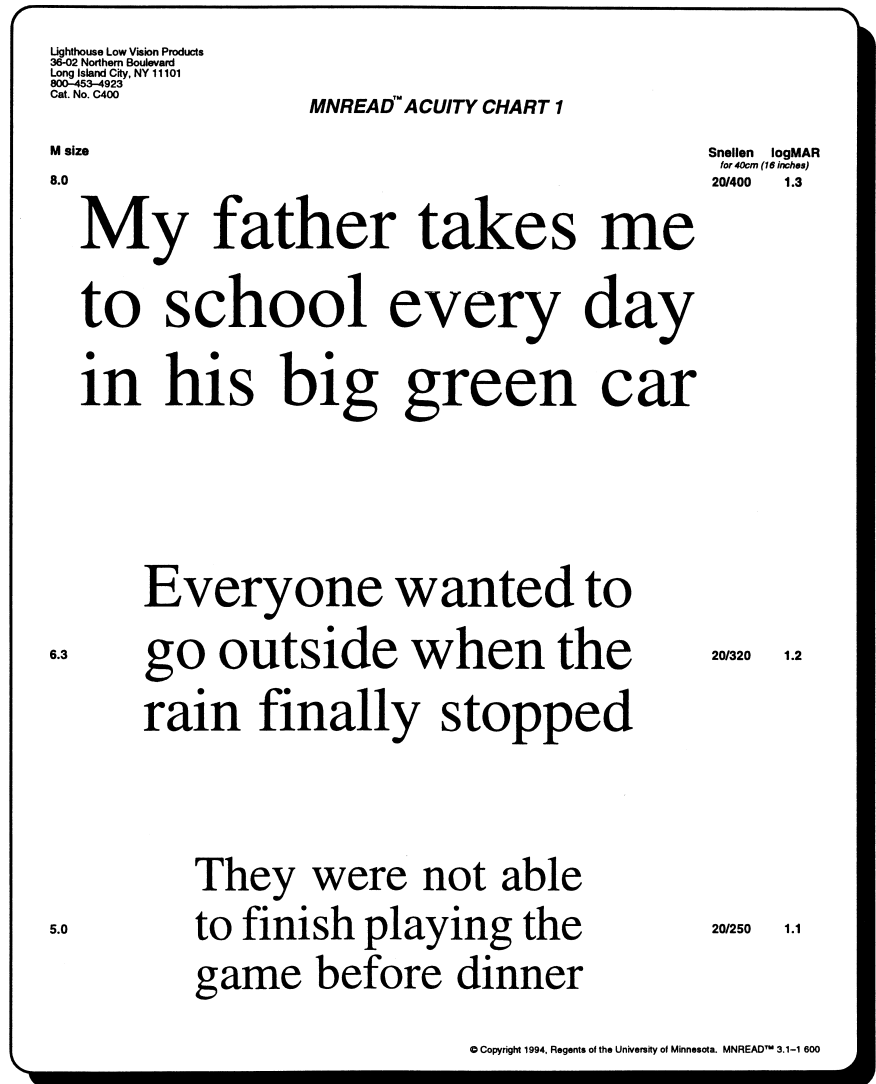
Fig. 1. Illustration of the MNREAD acuity chart. This chart is used for measuring three characteristics of reading vision: reading acuity, critical print size, and maximum reading speed.
